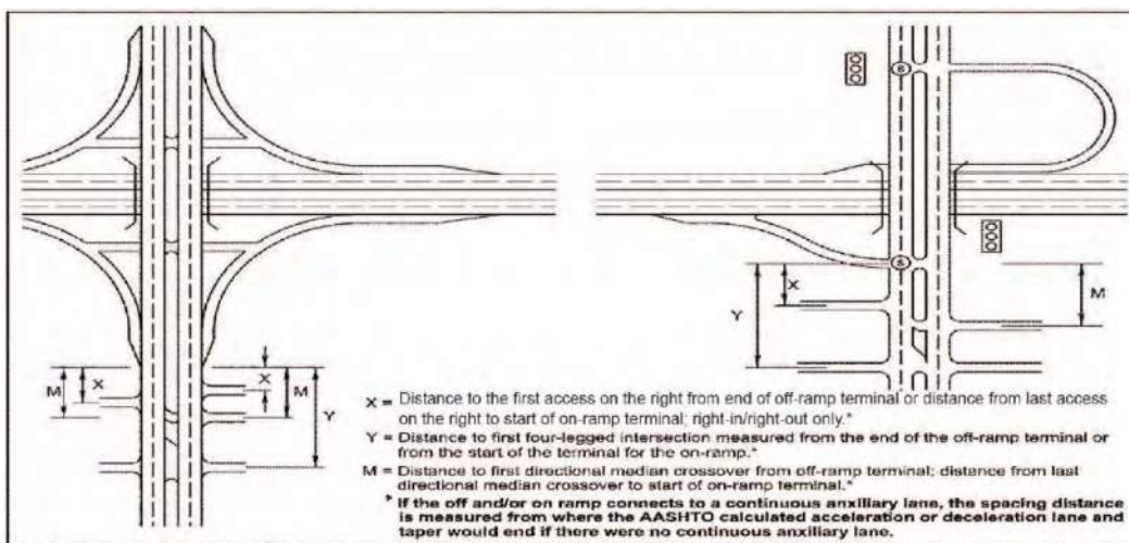
FIGURE 2-9 ACCESS CONTROL ON MULTILANE CROSSROADS AT INTERCHANGES
