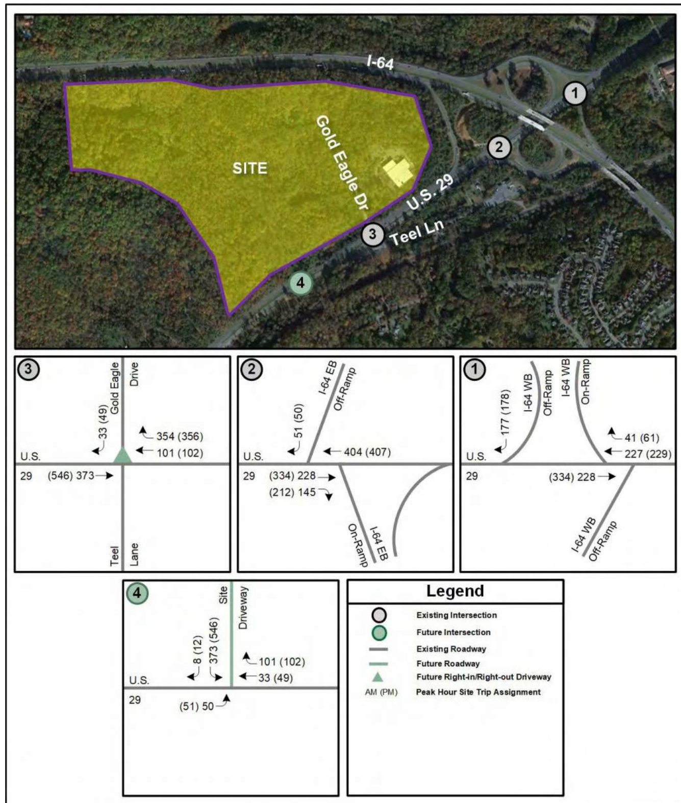
Figure 5: Primary Site Trip Assignment
