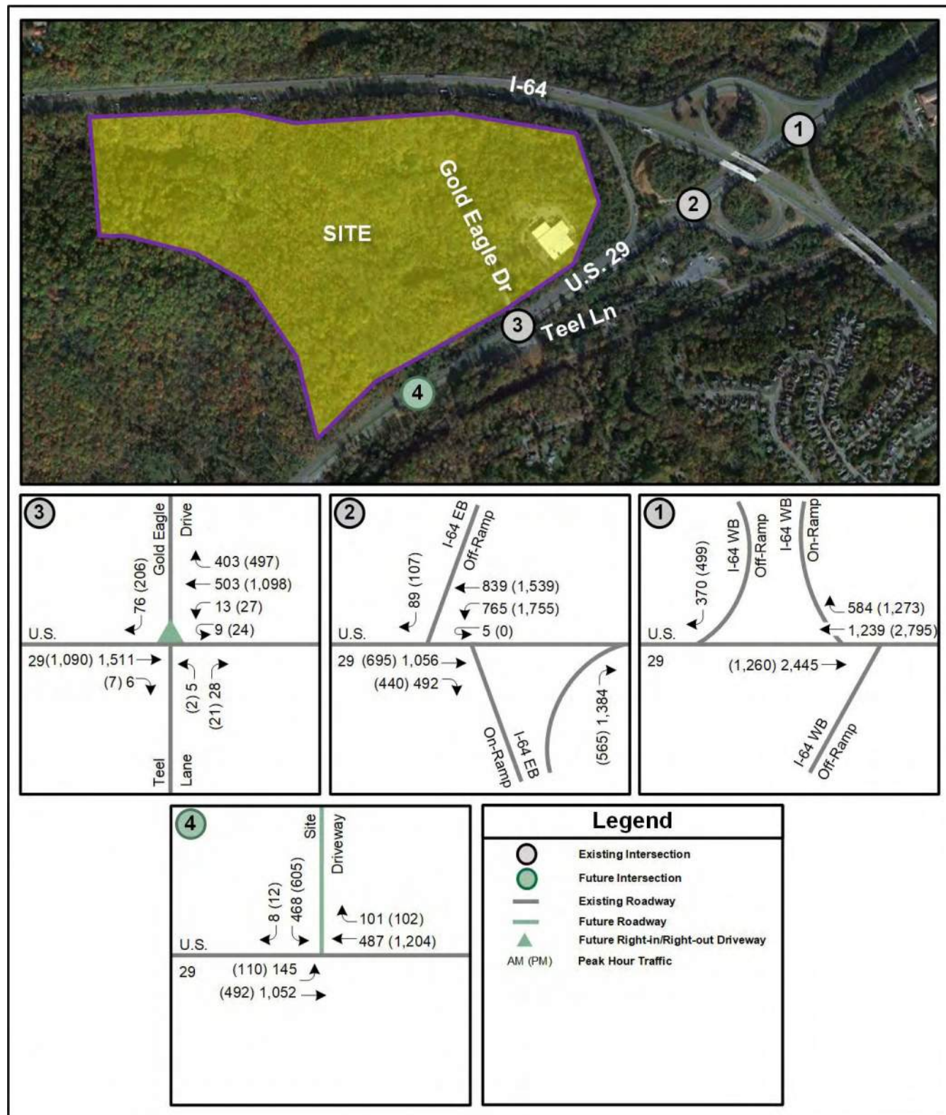
Figure 9: Build (2036) Peak Hour Traffic Volumes
