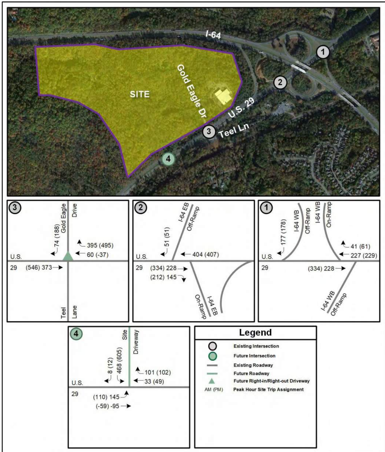
Figure 7: Total Site Trips
