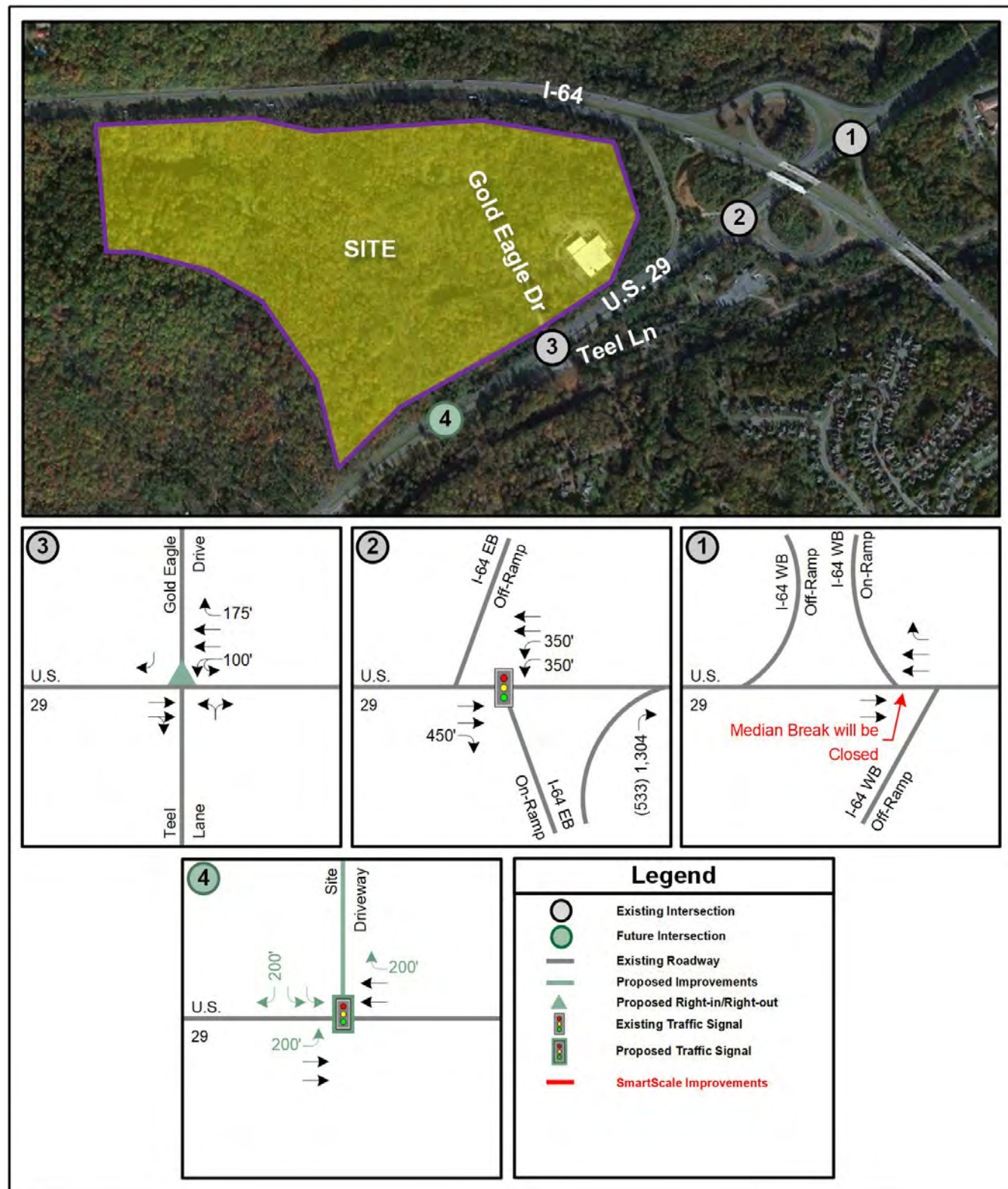
Figure 12: Recommended Lane Configuration
