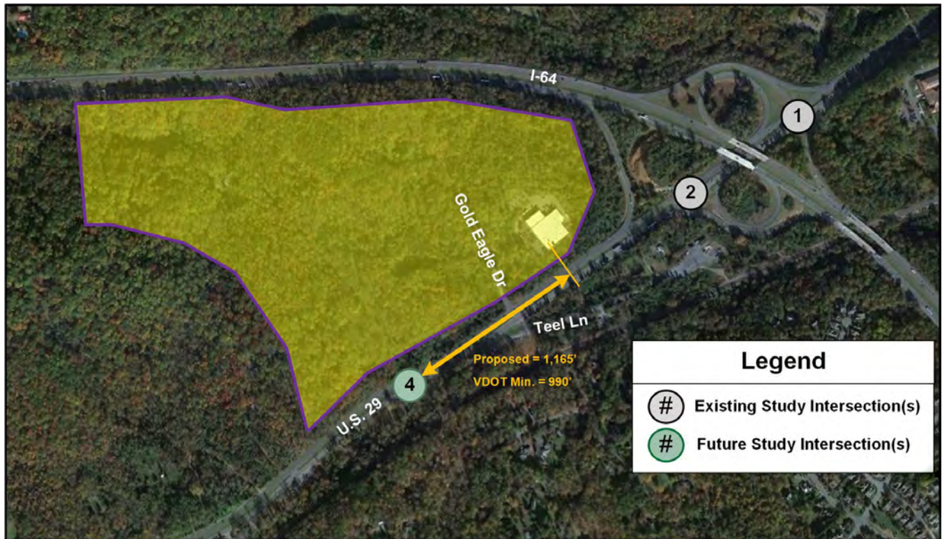
Figure 11: Proposed Intersection Spacing
